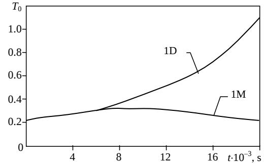
Fig. 4. Maximum temperature of fuel claddings T_0=T_0/T_{lim} in the reactor: 1D – DAMS, 1M – MAMS
