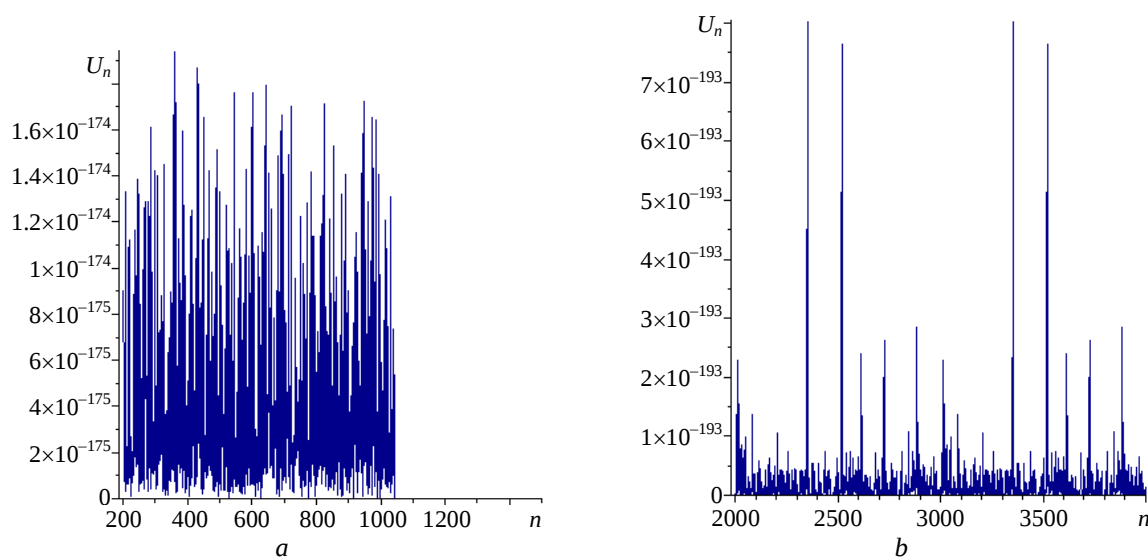
Fig. 4. Residual graphs U_n at different intervals of the variable n in the plane (n, U_n) : n \in [200, 1400] (a); n \in [2000, 4000] (b)
