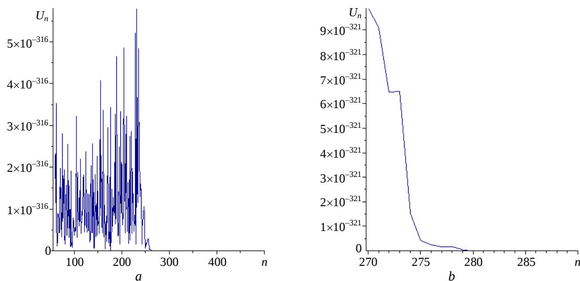
Fig. 8. Residual graphs U_n at different intervals of the variable n in the plane (n, U_n) : n \in [50, 500] (a); n \in [270, 290] (b)
