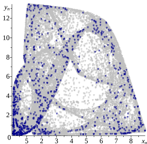
Fig. 11. 1001-cycle of the-system (13) in plane (x_n, y_n)
