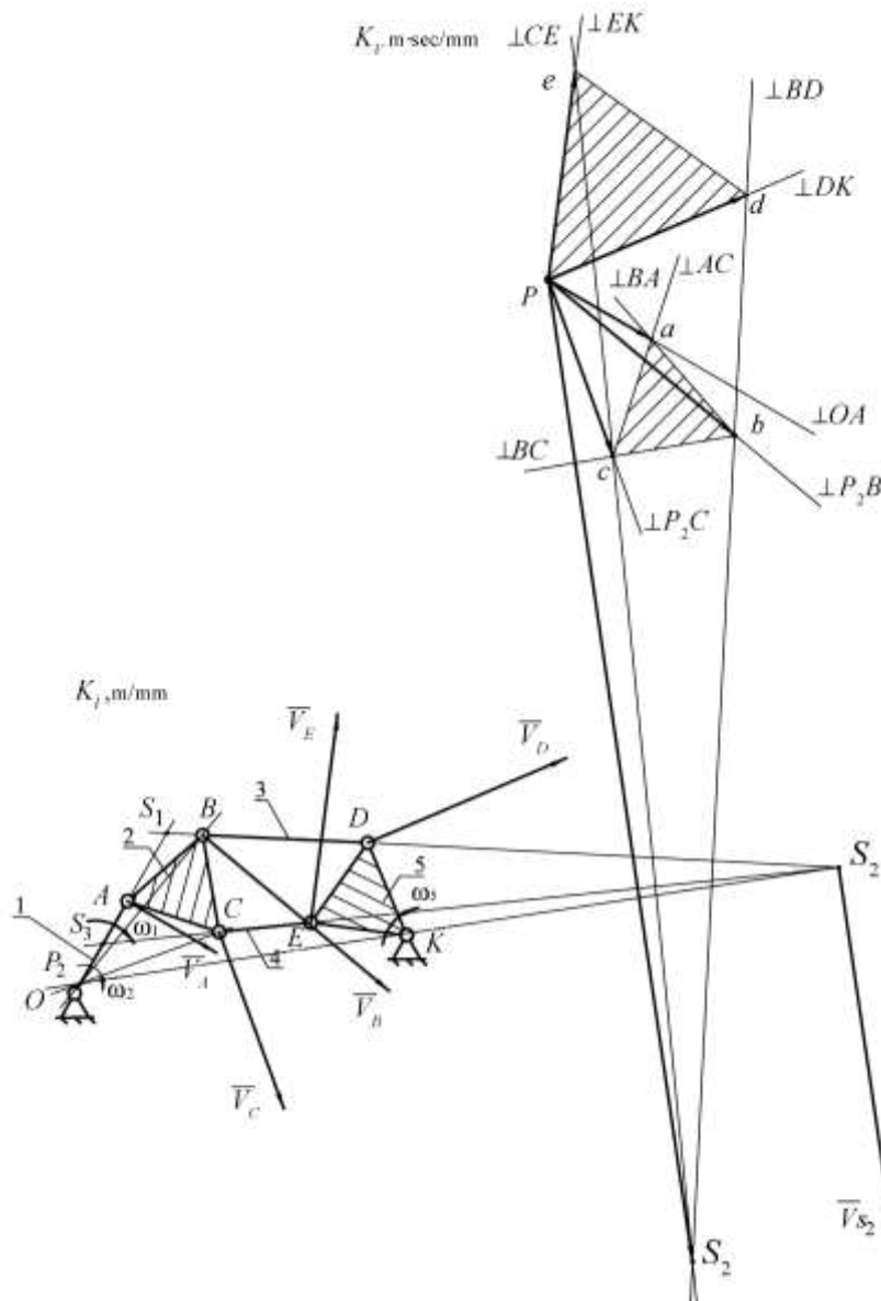
Fig. Kinematic scheme and velocity vector diagram of the fourth class mechanism
