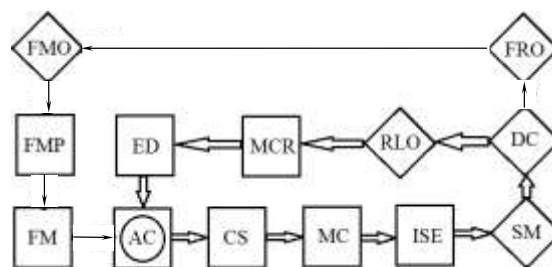
Block diagram of an automated system for control of VVER-1000 fuel properties: AC – active core; CS – core sensors; MC – marshalling cabinets; ISE – low-level and high-level equipment of the in-core instrumentation system; SM – simulation model for fuel performance optimization; DC – data comparator for analysis of cladding damage parameter values; RLO – block calculating the objective function for reactor loading optimization; MCR – main control room; ED – executive device for reactor power change; FRO – block calculating the objective function for fuel rearrangement optimization; FMO – block for fueling machine operation optimization; FMP – fueling machine control panel; FM – fueling machine
