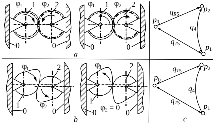
Fig. 3. Modeling of additional mechanical loops by kinematic orgraphs: with linear control function (a); with nonlinear control function (b); corresponding models in the form of kinematic orgraph (c)
