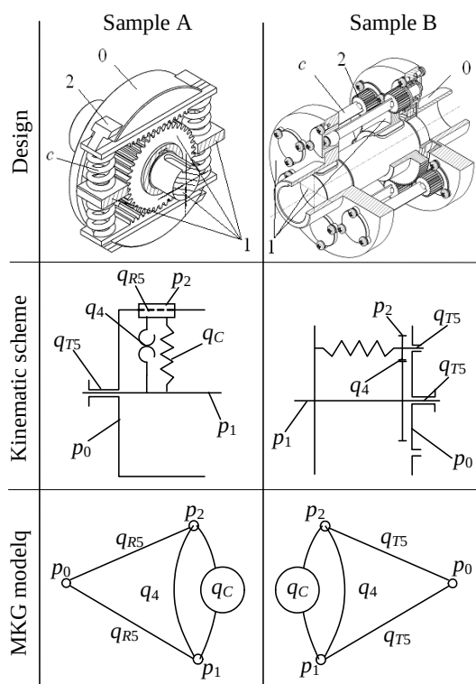
Fig. 1. Modeling of passive elastic couplings with linear mechanical feedback of modified kinematic graph (MKG)
