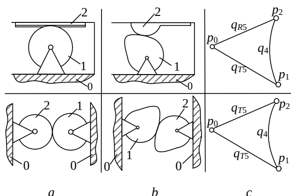
Fig. 2. Modeling of additional mechanical loops by kinematic graphs: with linear control function (a); with nonlinear control function (b); model in the form of kinematic graph (c)
