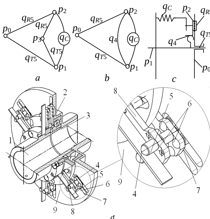
Fig. 5. Synthesis of structure of elastic coupling with nonlinear mechanical feedback and its constructive realization
