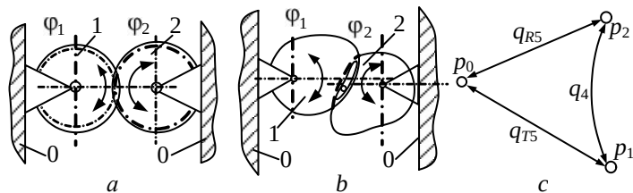
Fig. 4. Modeling of additional mechanical loops by kinematic orgraphs: with linear control function (a); with nonlinear control function (b); corresponding models in the form of kinematic orgraph (c)
