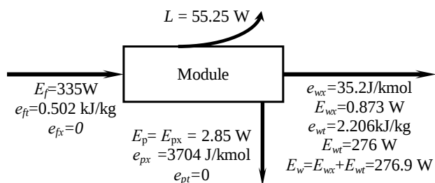
Fig. 3. Scheme of exergy flows in reverse osmosis module
