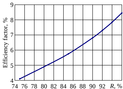
Fig. 6. Dependence of exergy efficiency factor on membrane selectivity R
