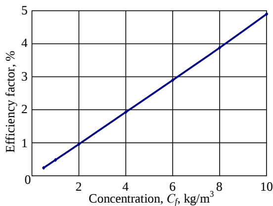
Fig. 5. Dependence of exergy efficiency factor on source water concentration
