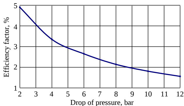
Fig. 4. Dependence of exergy efficiency factor on drop of pressure
