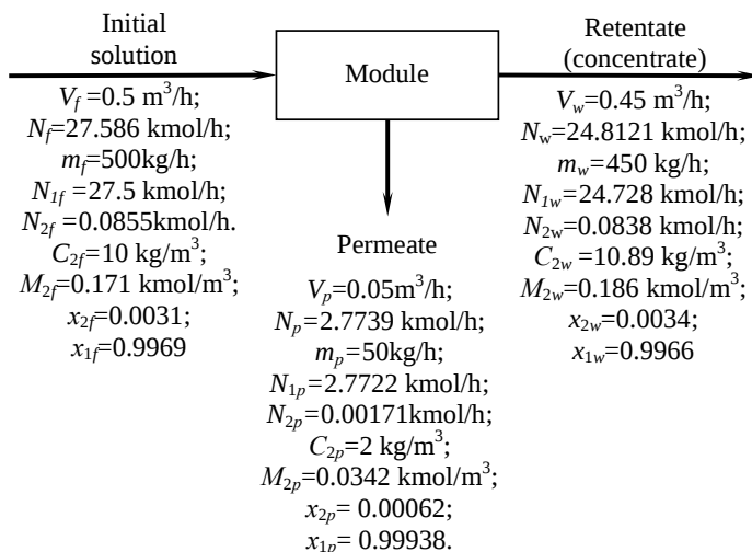
Fig. 1. Material balance of osmotic module
