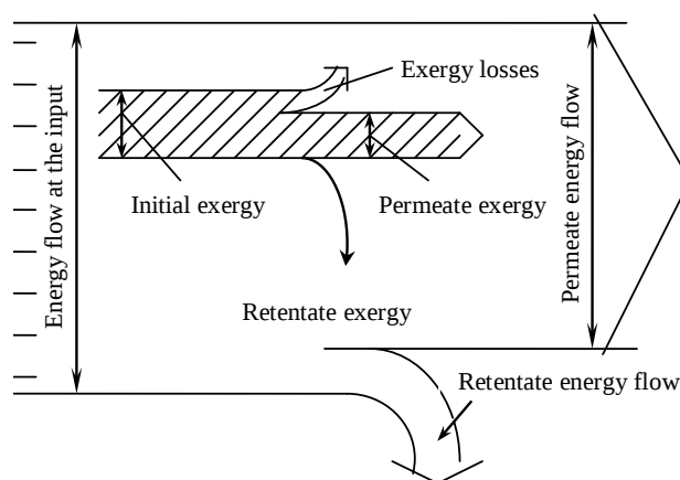
Fig. 2. Scheme of energy and exergy flows in reverse osmosis module
