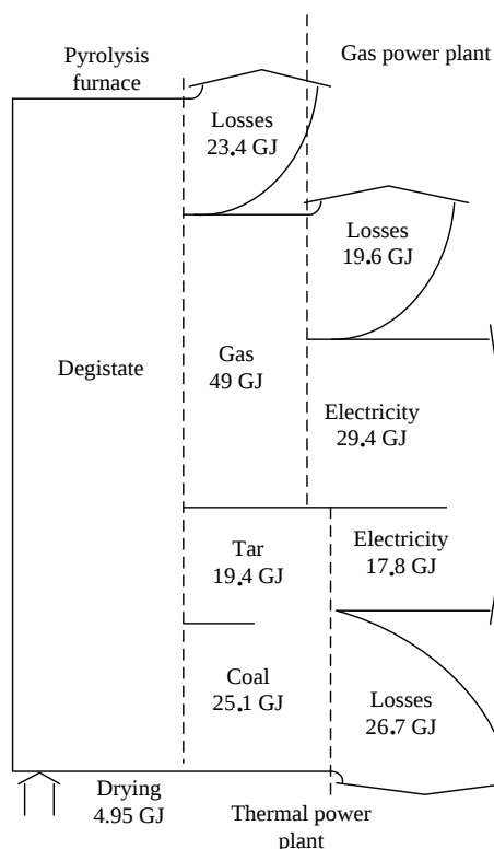
Fig. 3. Diagram of energy flows in a pyrolysis plant
