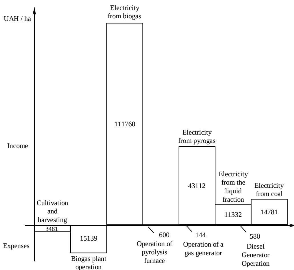
Fig. 4. Cost-benefit ratio in biogas digesters deep processing technology
