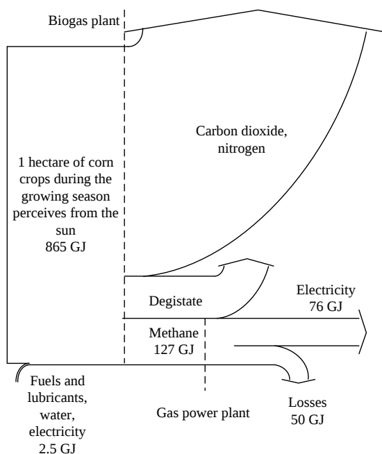
Fig. 2. Diagram of energy flows in a biogas digester
