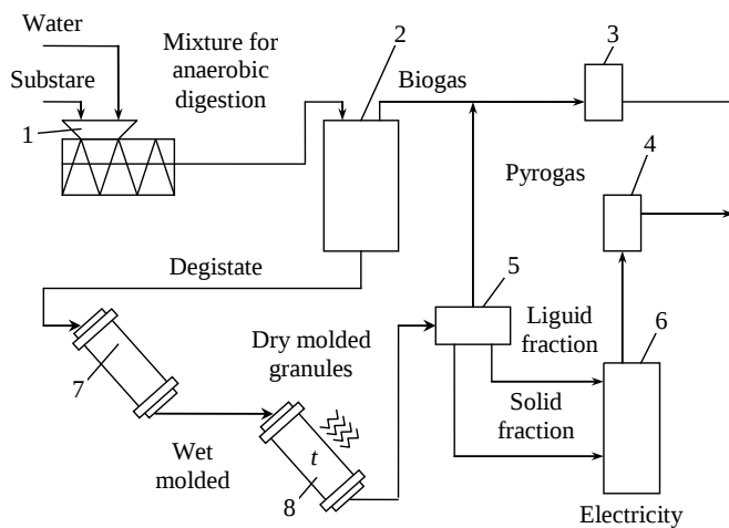
Fig. 1. General structural scheme of cogeneration complex of deep digestate processing: screw mixer (1); reactor-methanogenic (2); gas generator (3); electric generator on black oil (4); pyrolysis furnace (5); module for the production of heating oil (a substitute for fuel oil) (6); drum granulator (7); drum dryer (8)
