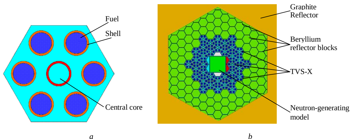
Fig. 2. Design model for determining fuel pellet enrichment: TVS-X (a); SI (b)
