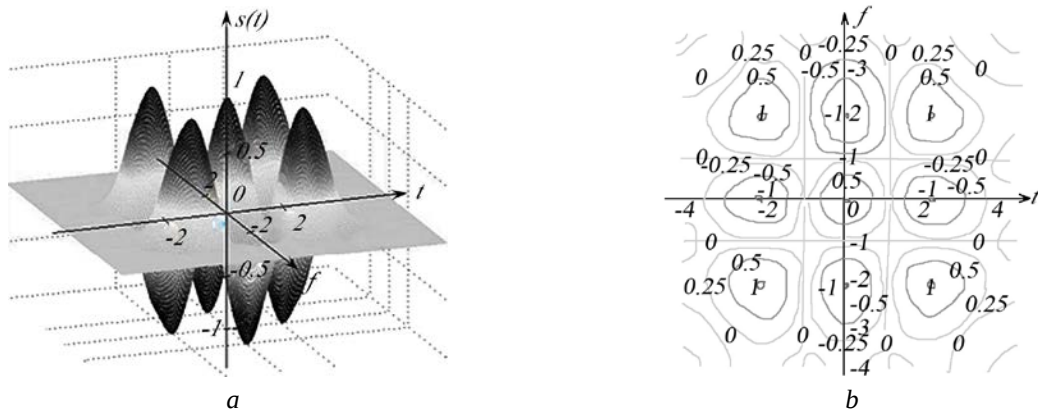
Fig. 1. Distribution of IOTA basis functions in time-frequency plane in OFTDM system: IOTA basis function (a), contour graph (b)
