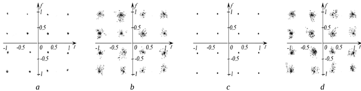
Fig. 2. Signal constellation for QAM-16 modulation: half cosine function (a), half cosine function with frequency shift (b), extended Gaussian function (c), extended Gaussian function with frequency shift (d)
