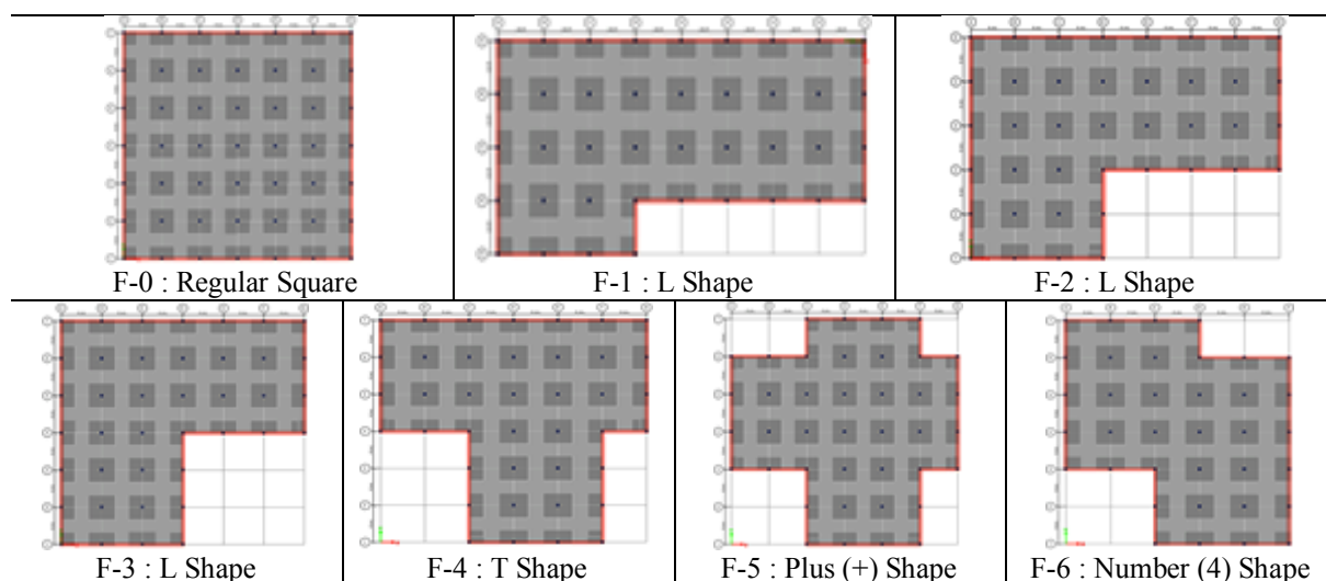
Plan shapes of analyzed buildings
