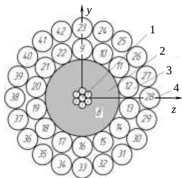
Fig. 2. Cable KOBDF-6 cross-section: 1 – conducting core; 2 – insulating layer; 3 – internal layer of armor; 4 – external layer of armor
