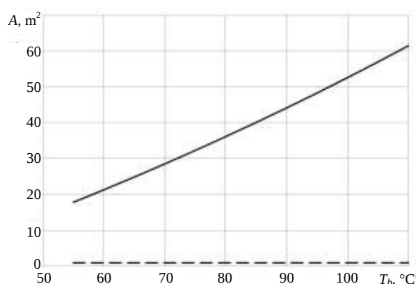
Fig. 6. The necessary surfaces areas of heat exchange for preliminary heaters of seawater:
