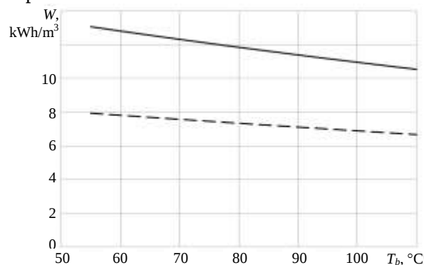
Fig. 4. Dependence of specific power consumption on temperature of seawater boiling at two various values of heat-transfer coefficient in evaporator-condenser: «—» — U_e = 2,5 \text{ kW}/(\text{m}^2 \cdot \text{K}) ; «---» — U_e = 5,0 \text{ kW}/(\text{m}^2 \cdot \text{K})
