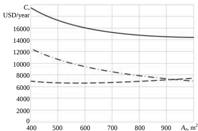
Fig. 7. The given annual costs as function of the surface area of heat exchange of evaporator-condenser: «—» — total annual costs; «---» — reduced capital costs; «- • -» — the annual cost of electricity
