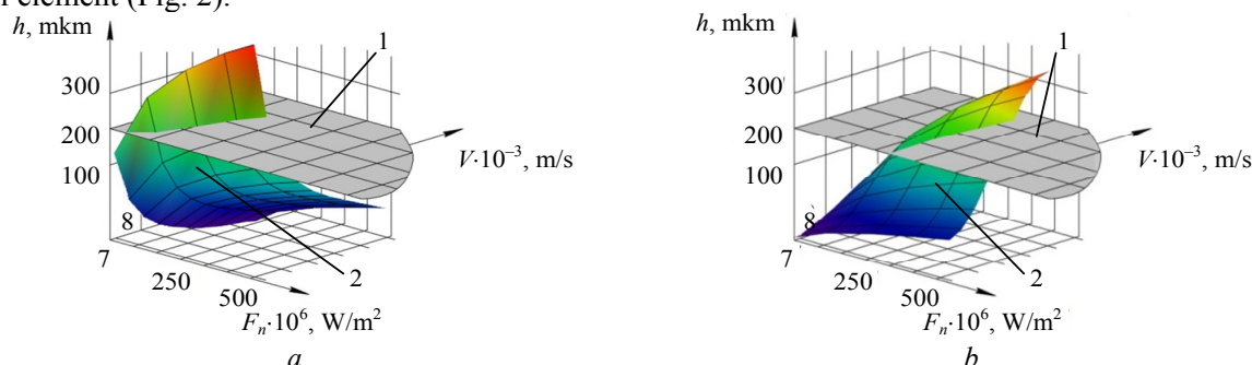
Fig. 2. Dependencies h_m(F_n, V) for elements of the optical glass K8 (a) and K108 (b):
