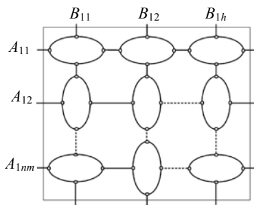
Fig. 17. Packed planar frame model of the switching matrix on the SEB \underline{B}^\#
