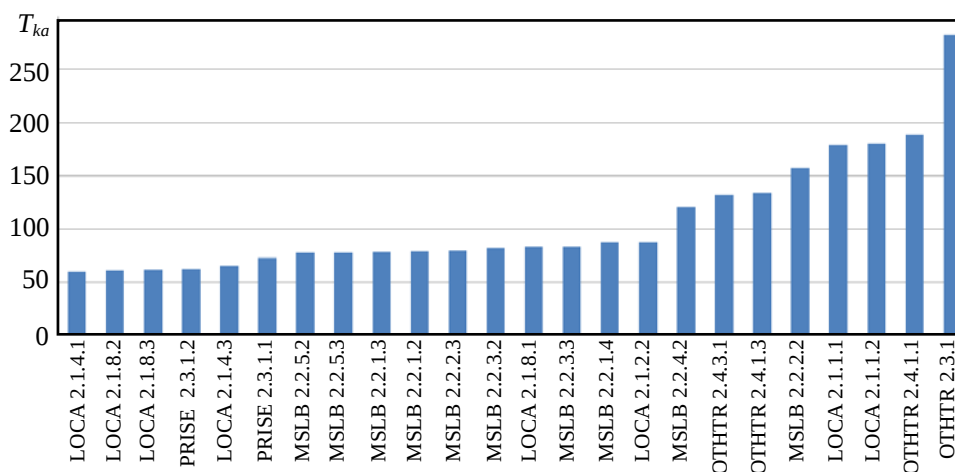
Fig. 2. Margin to brittle strength ( T_{ka} ), the second part of the scenarios
