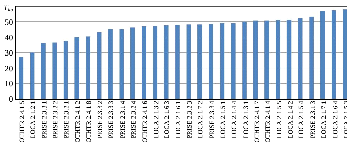
Fig. 1. Margin to brittle strength ( T_{ka} ), the first part of the scenarios
