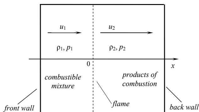
Fig. 1. Scheme of flame in closed fire-chamber, tube or channel
