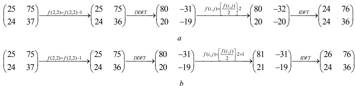
Fig. 1. Steganographic algorithm based on DFT to block 2 \times 2 the embedding of AI in the integer frequency coefficients DFT: insert (a) 0; insert 1 (b)
