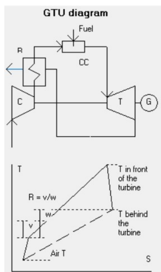
Fig. 5. Scheme of a gas turbine installation with heat regeneration without its utilization
