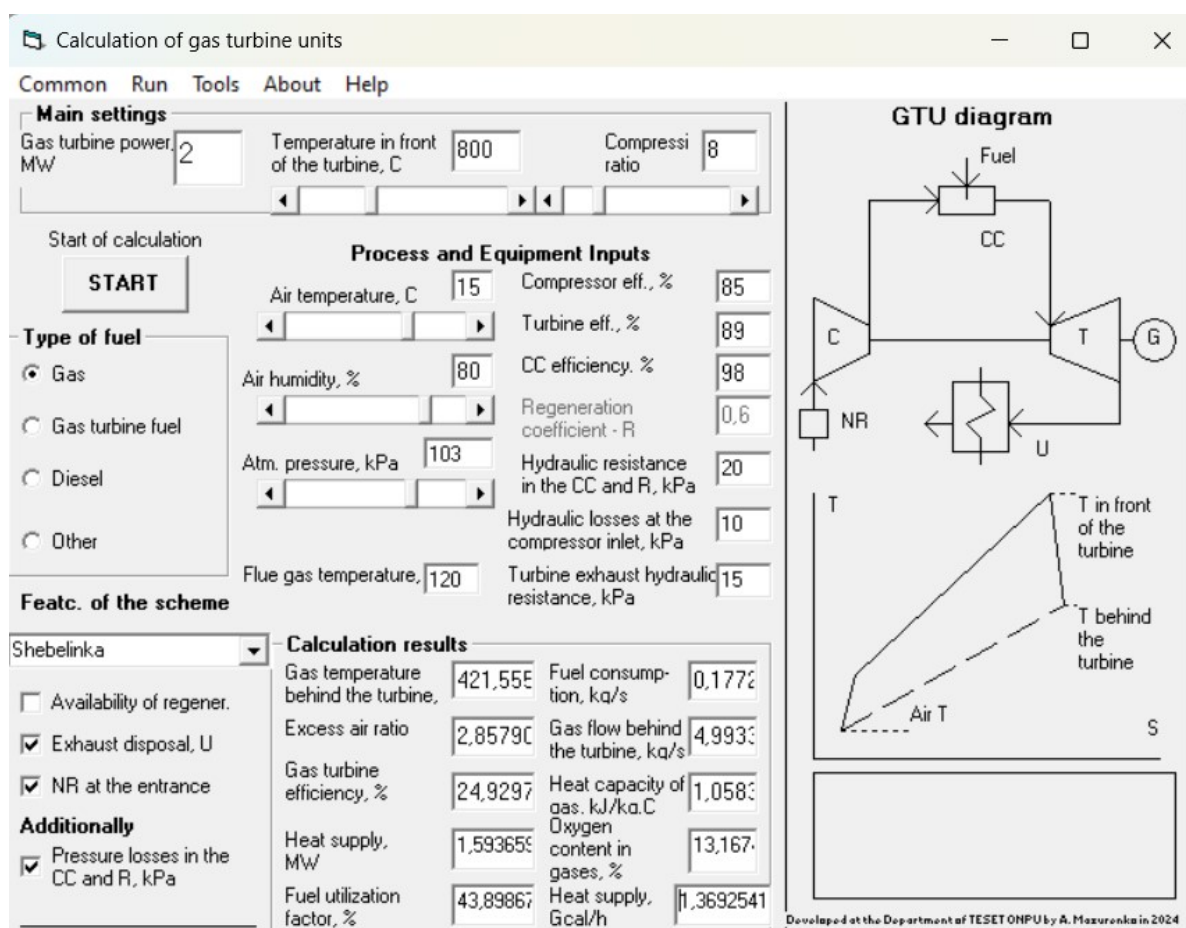
Fig. 4. Working window of the program for calculations and analysis of the gas turbine installation in the heat supply system
