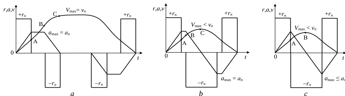
Fig. 1. Optimal diagrams of the elevator car movement at different distances of its movement: trapezoidal acceleration diagram (a); truncated trapezoidal acceleration diagram (b); triangular acceleration diagram (c)
