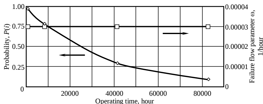
Fig. 4. Probability of failure-free operation of the NWT-3 system
