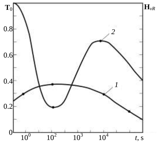
Fig. 2. Maximum temperature of fuel claddings and the coolant level in the reactor for MAMS with LLOCA and blackout: 1 – T_0 = T_0/T_{lim} , 2 – H_{vR} = H_{vR}/H_{vR0}
